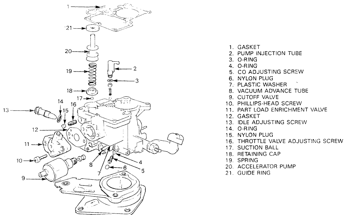
Figure 4 Carburetor body
