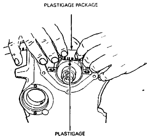
Figure 24 Measurement of crankshaft bearing clearance
