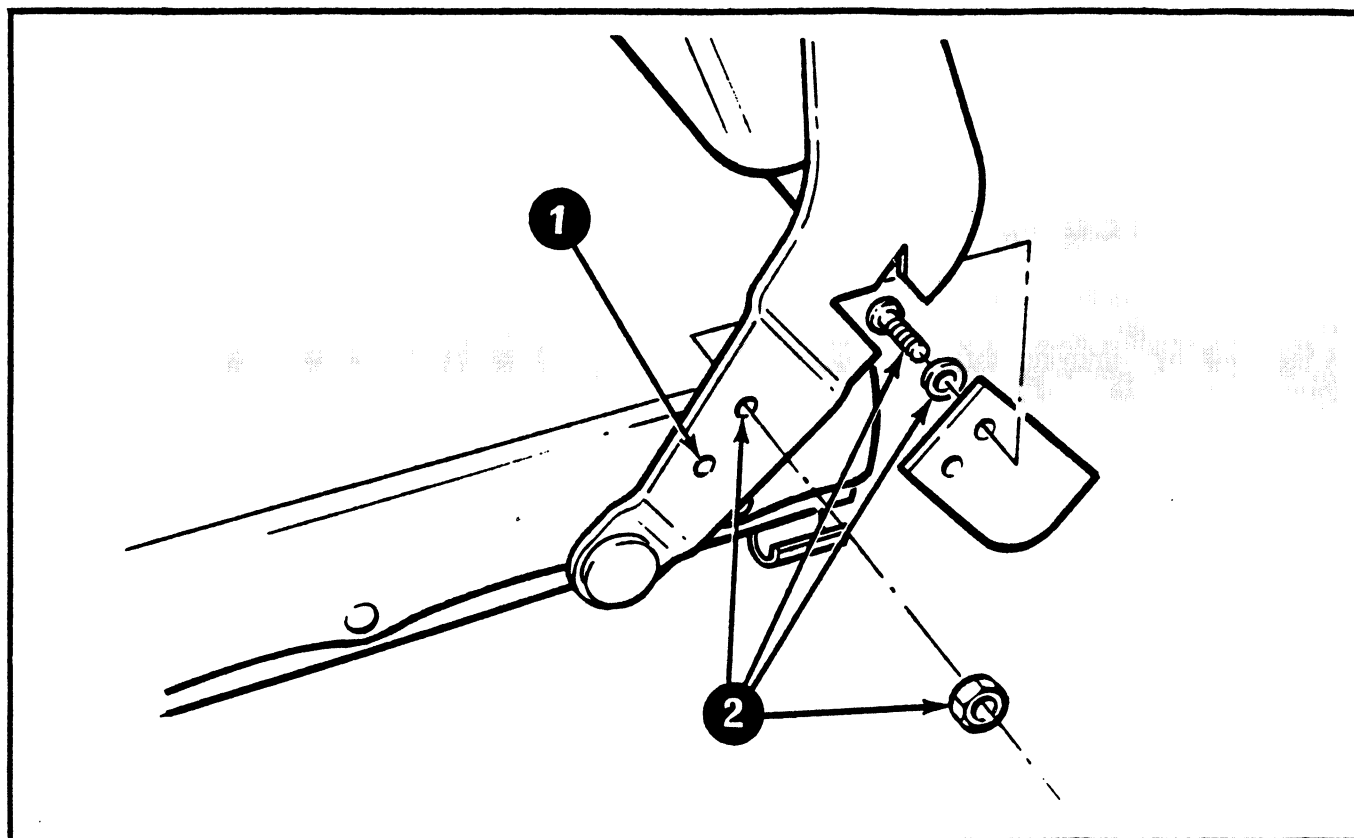
Figure 3-3 Installation of Rear Seat Stand-Off Brackets
