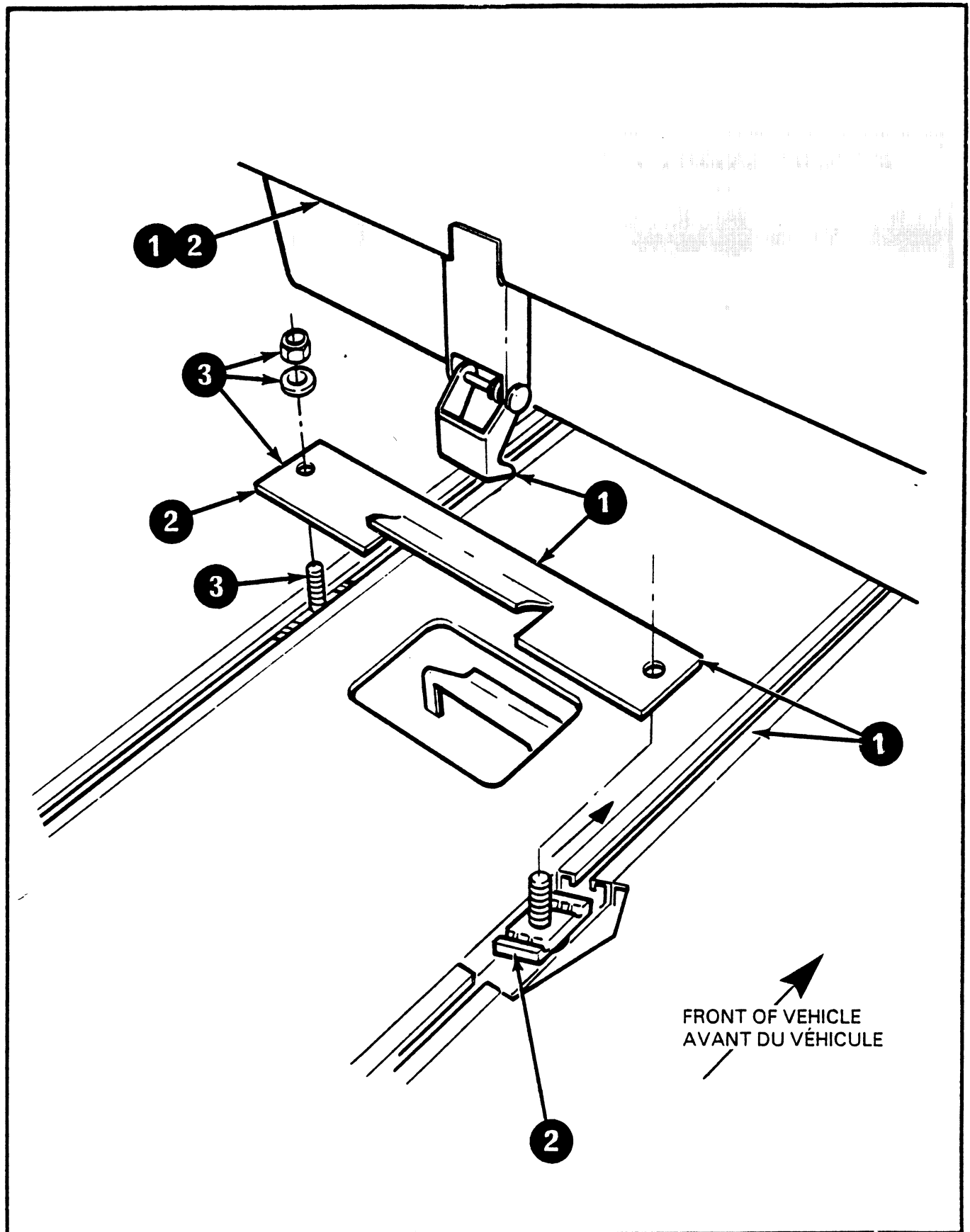
Figure 3-4 Installation of Seat Catch Brackets
