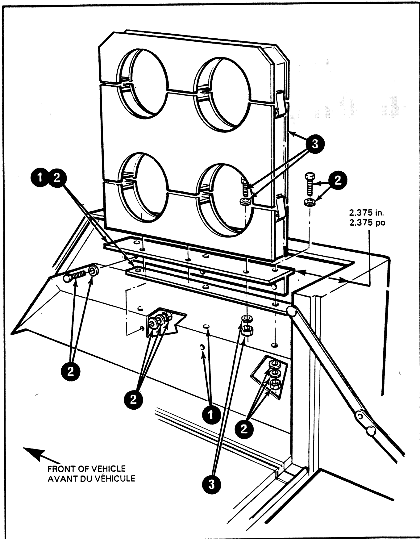
Figure 3-5 Installation of Iltis TOW 2 Stowage Rack Assemblies
