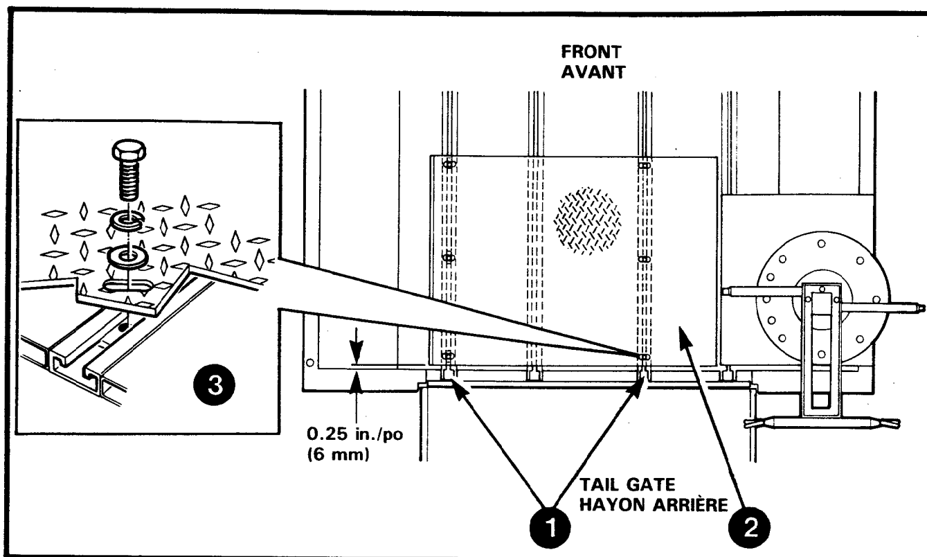
Figure 3-9-2 Installation of Floor Plate
