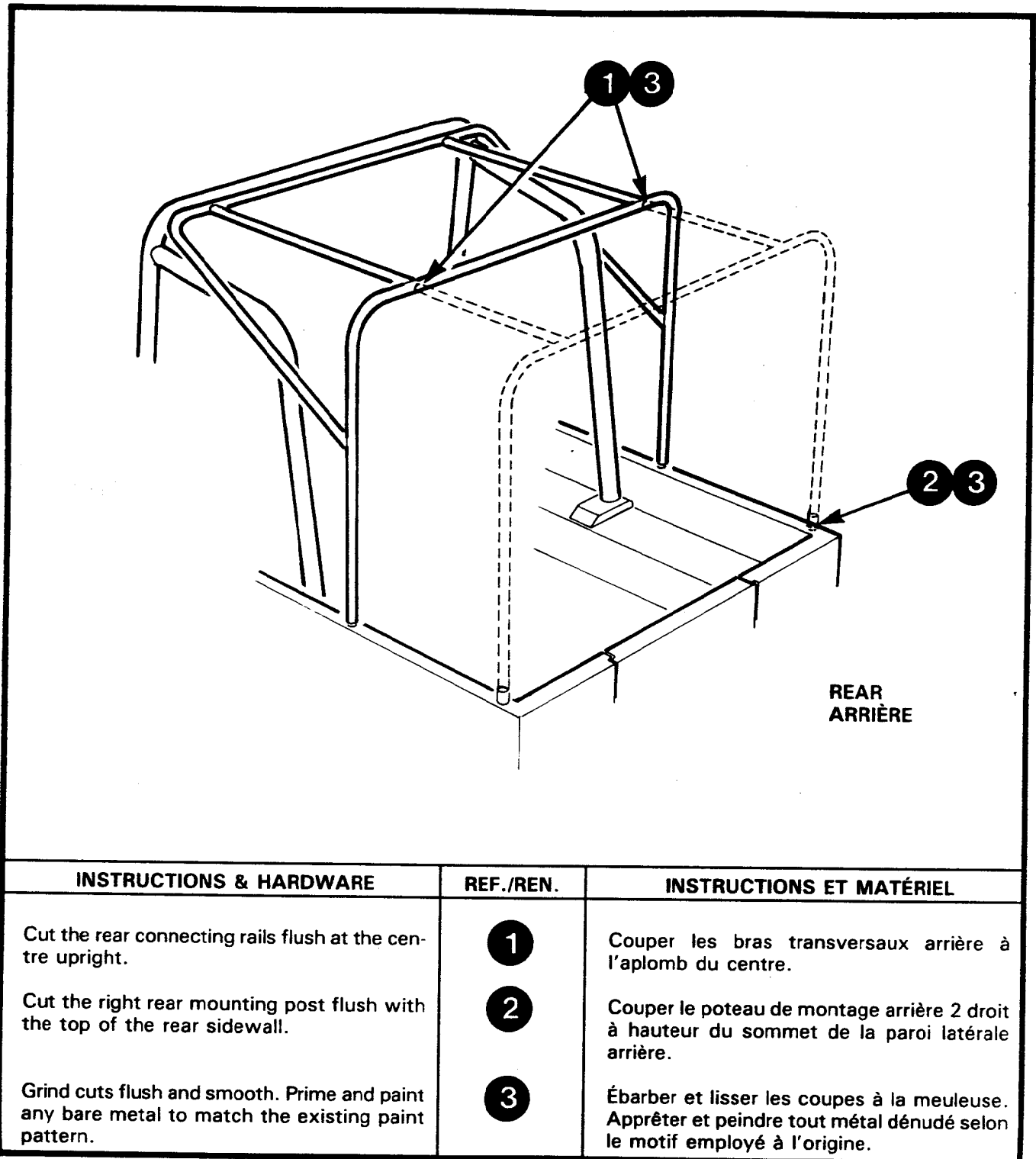
Figure 2-2 Preparation of Superstructure Figure 2-2 Préparation de la superstructure
