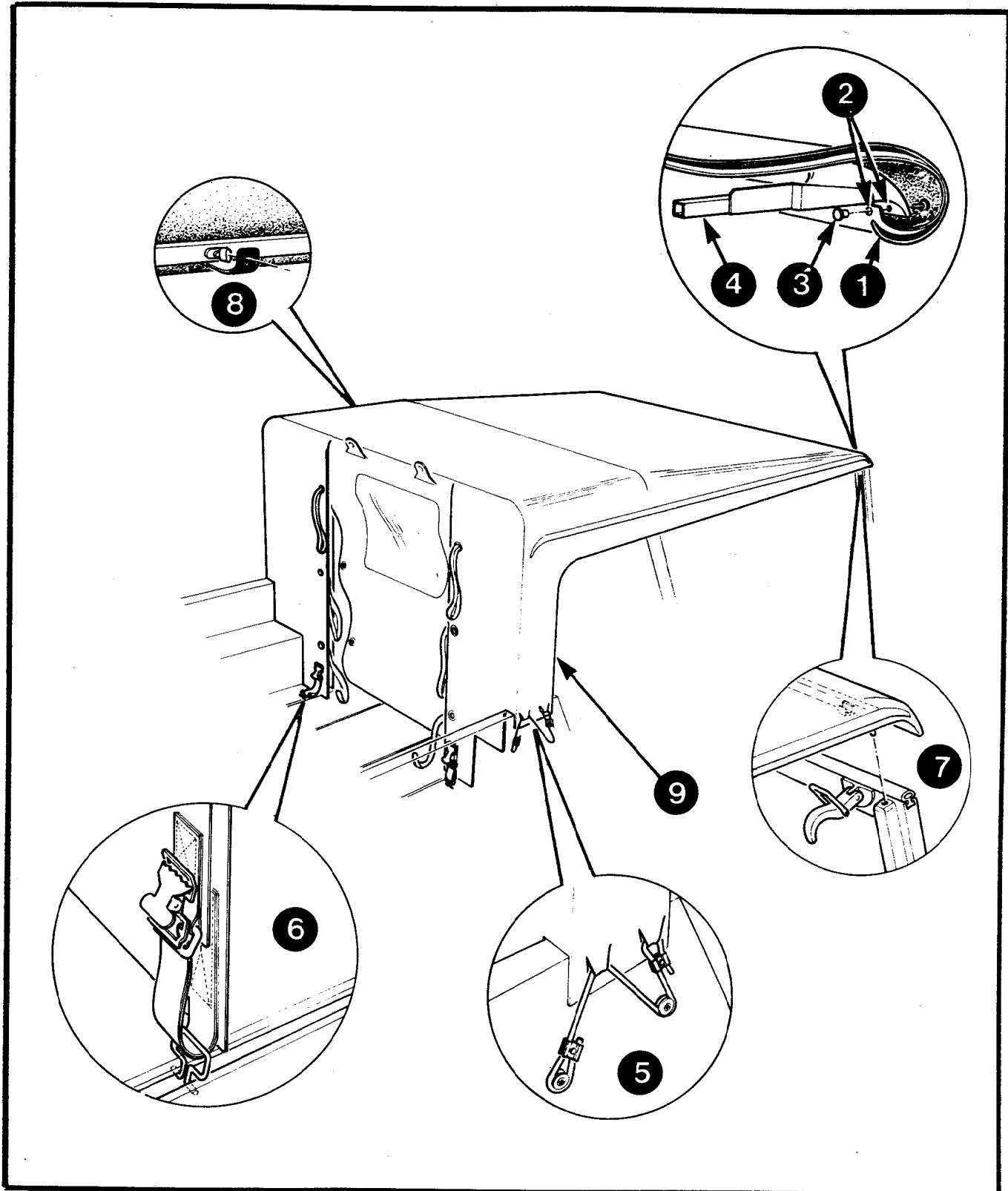
Figure 3-12-2 Installation of the Tarpaulin
