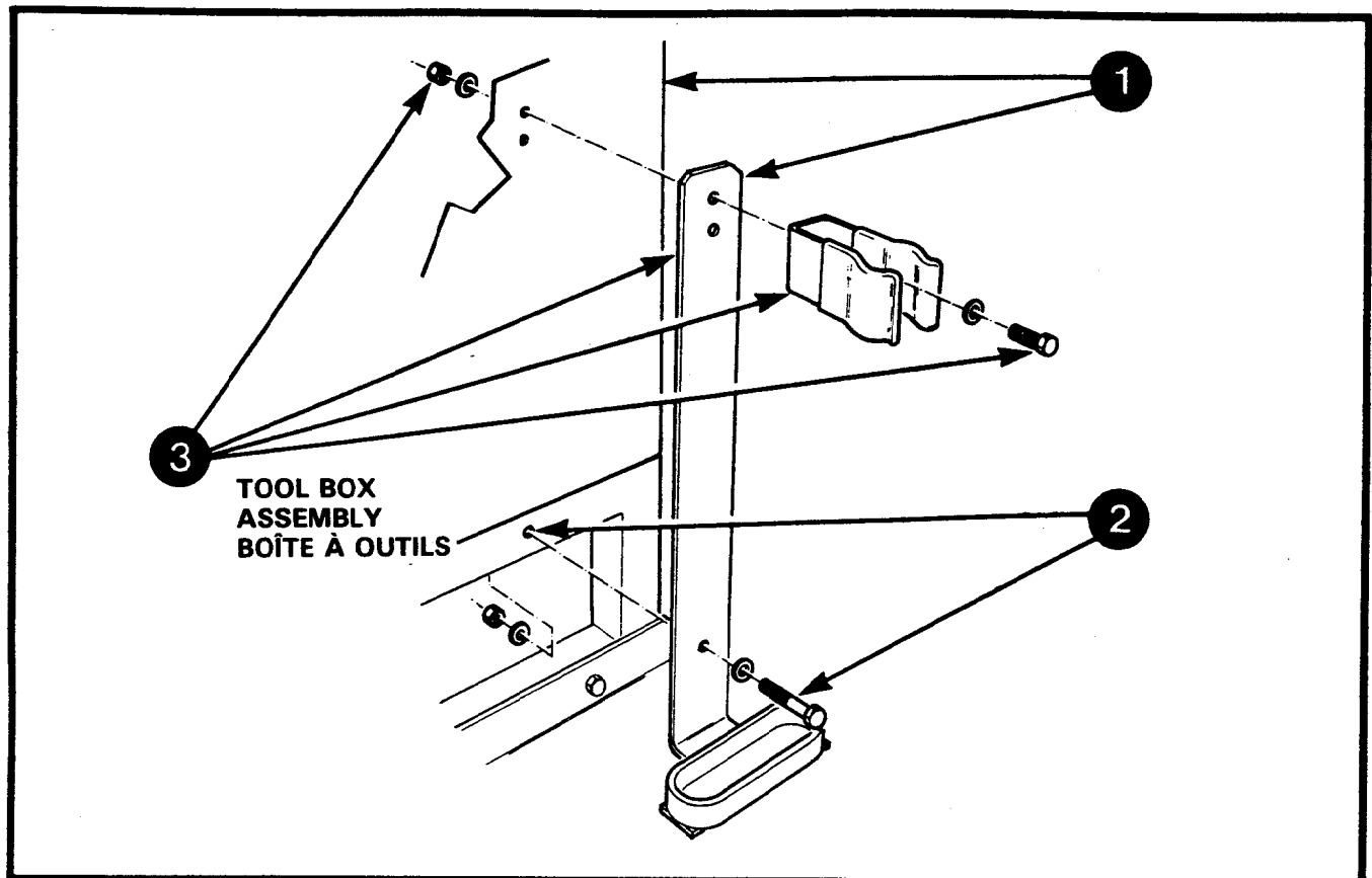
Figure 3-11-2 Installation of Weapon Mount
