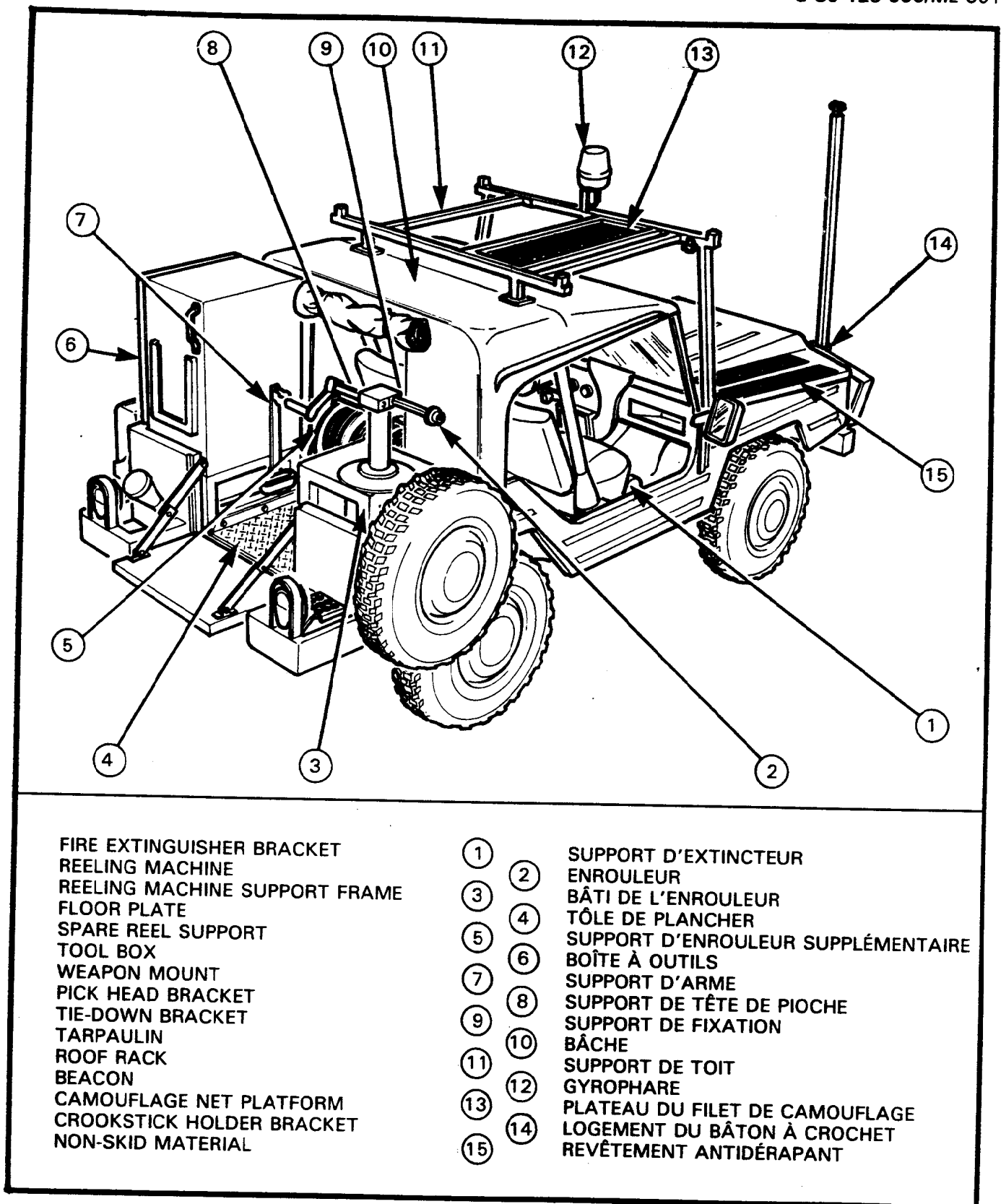
Figure 1-1 Primary Components of the Ilitis Cable Laying Kit
