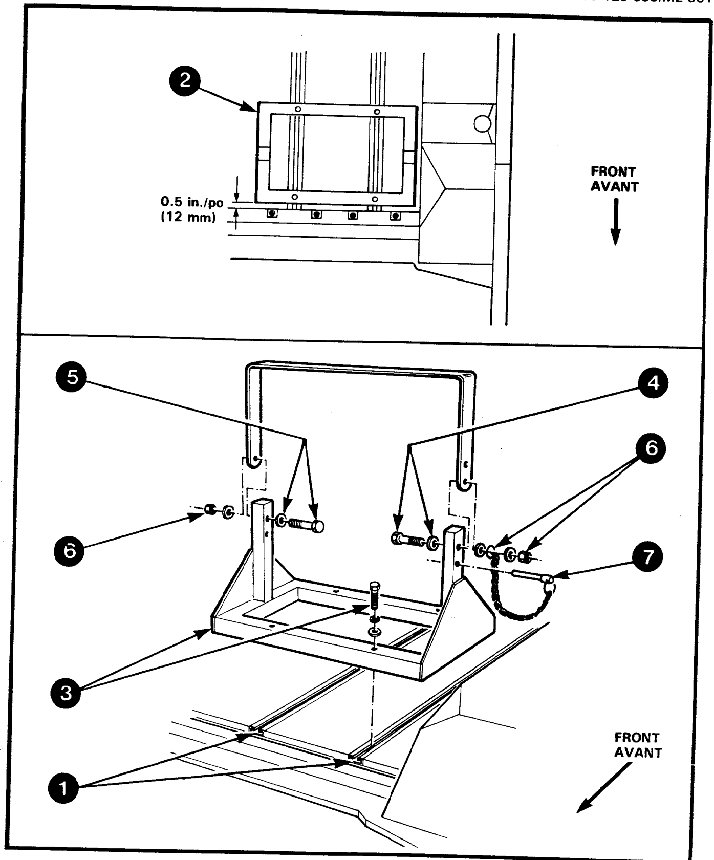
Figure 3-4-2 Installation of Spare Reel Support
