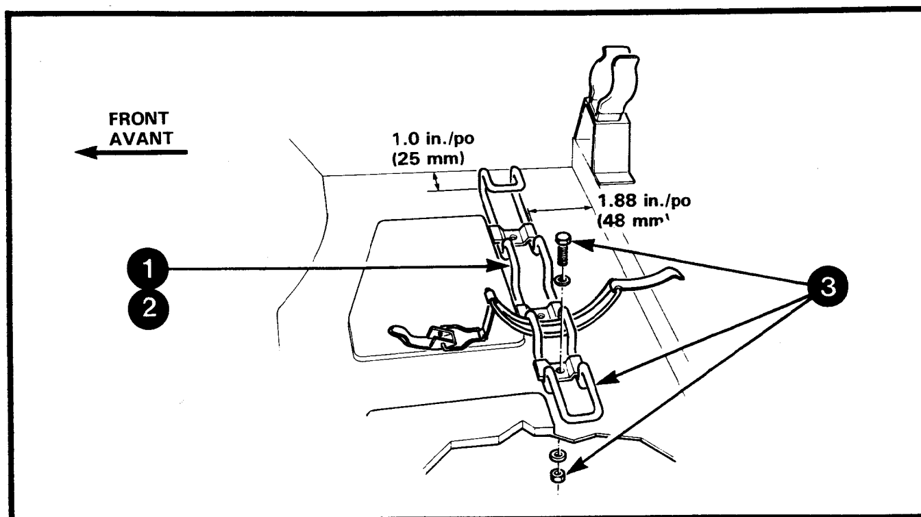
Figure 3-2-2 Installation of Fire Extinguisher Bracket
