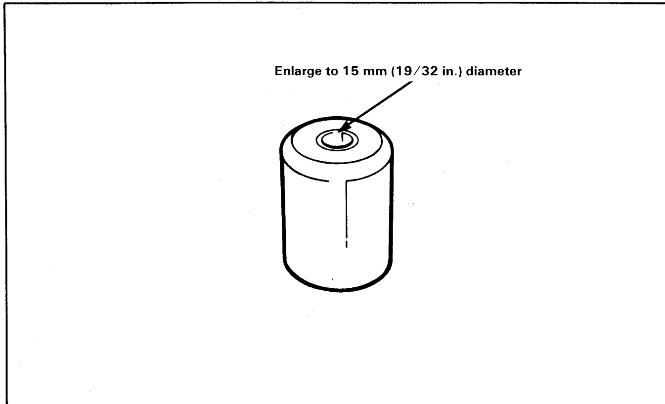
Figure 1 Enlarge Sleeve Hole of Special Tool
