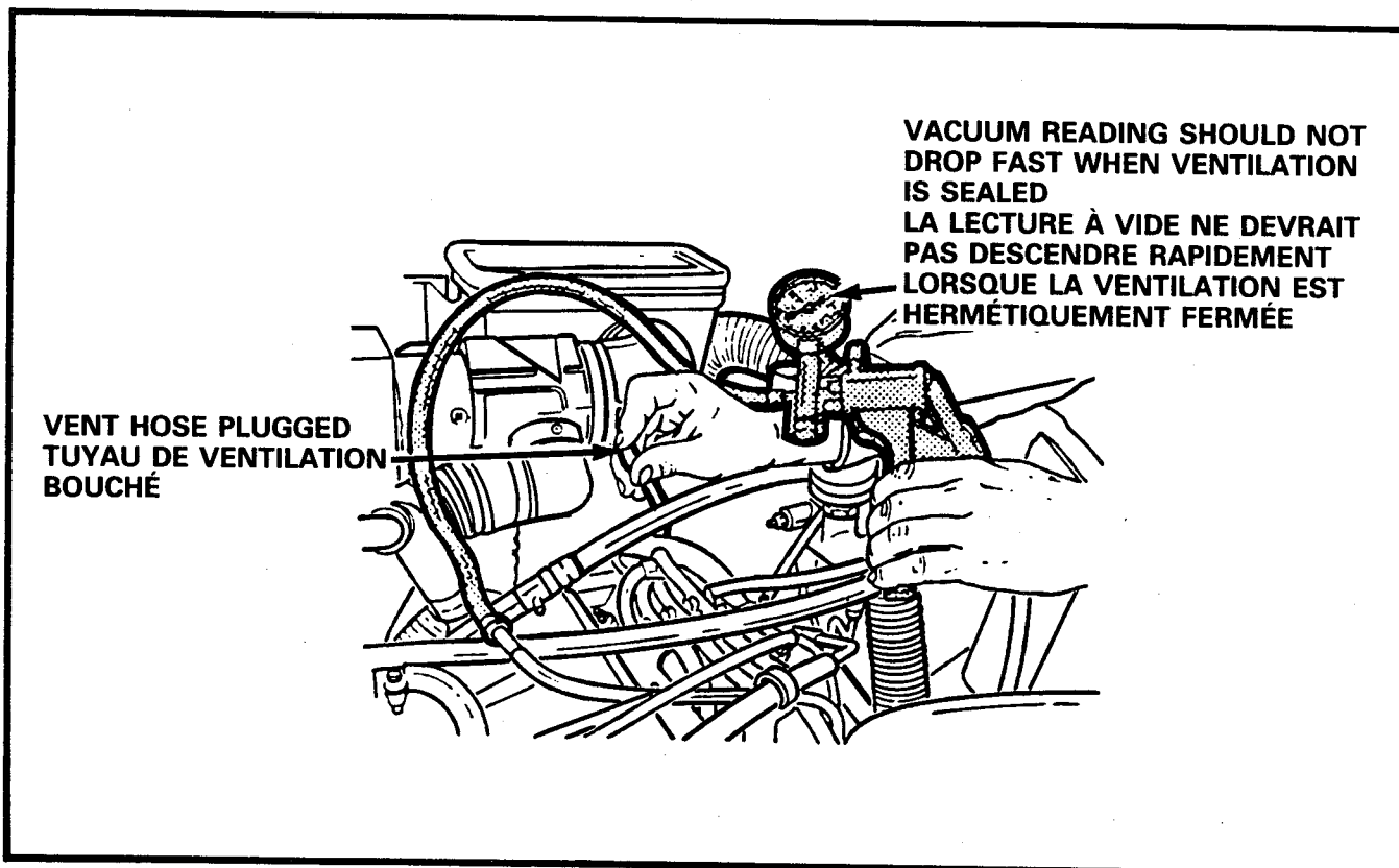
Figure 2 Checking For Leakage and For Free Operating Mechanism
