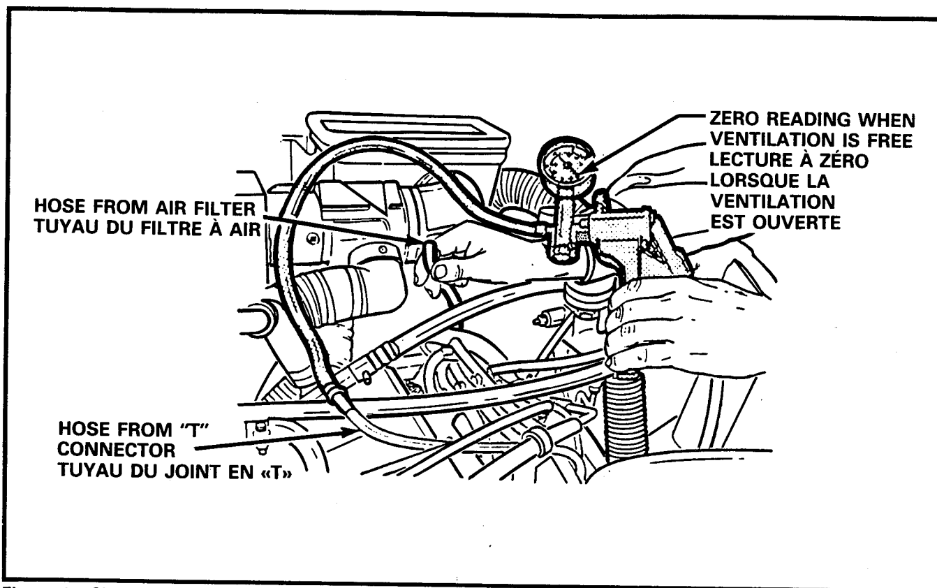
Figure 1 Checking For Clogged Distributor
